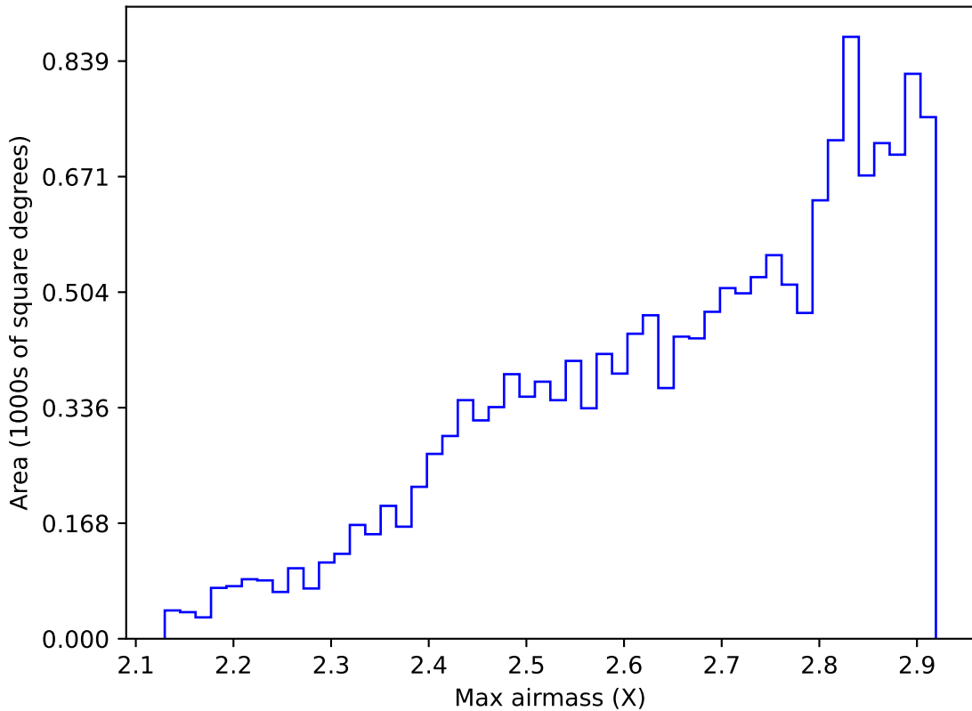
too_ignore_100_4v3.4_10yrs WFD all bands: Max airmass
