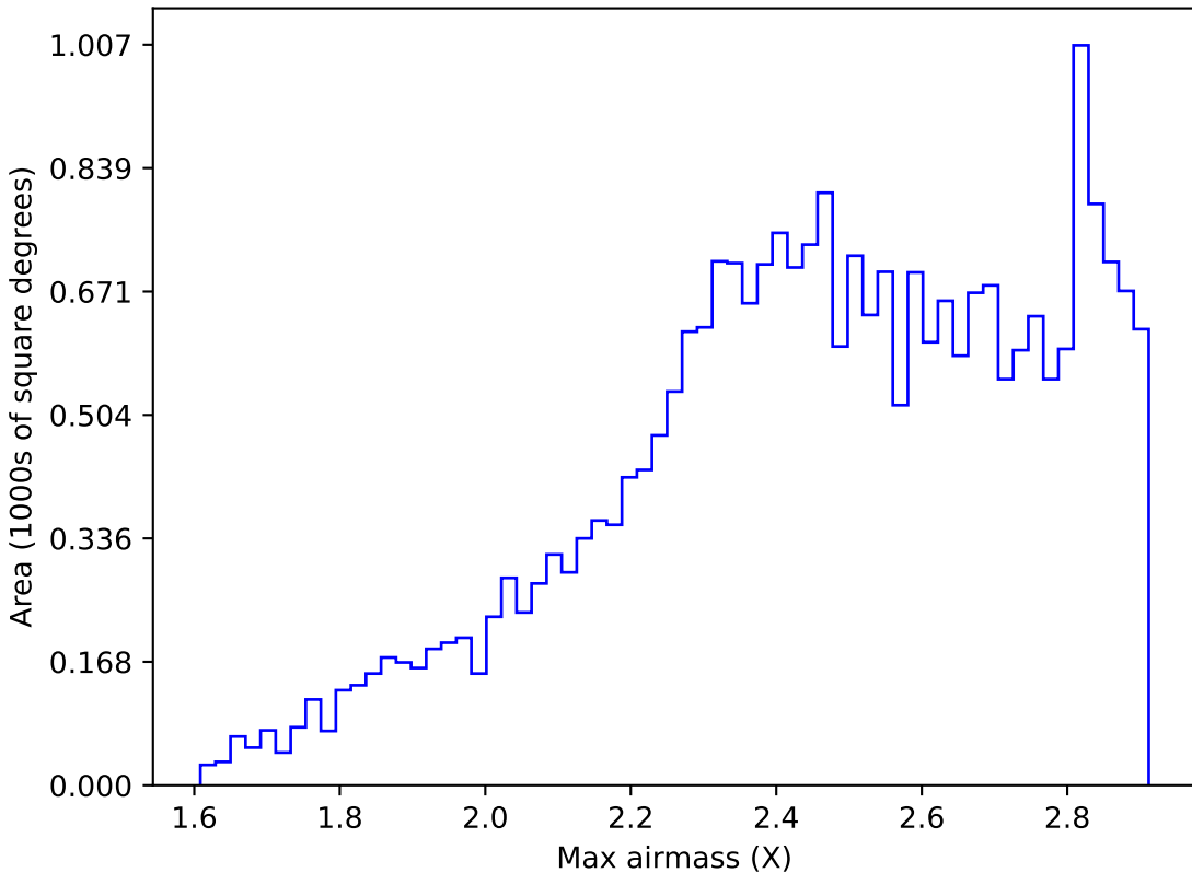
too_ignore_100_4v3.4_10yrs All sky z band: Max airmass
