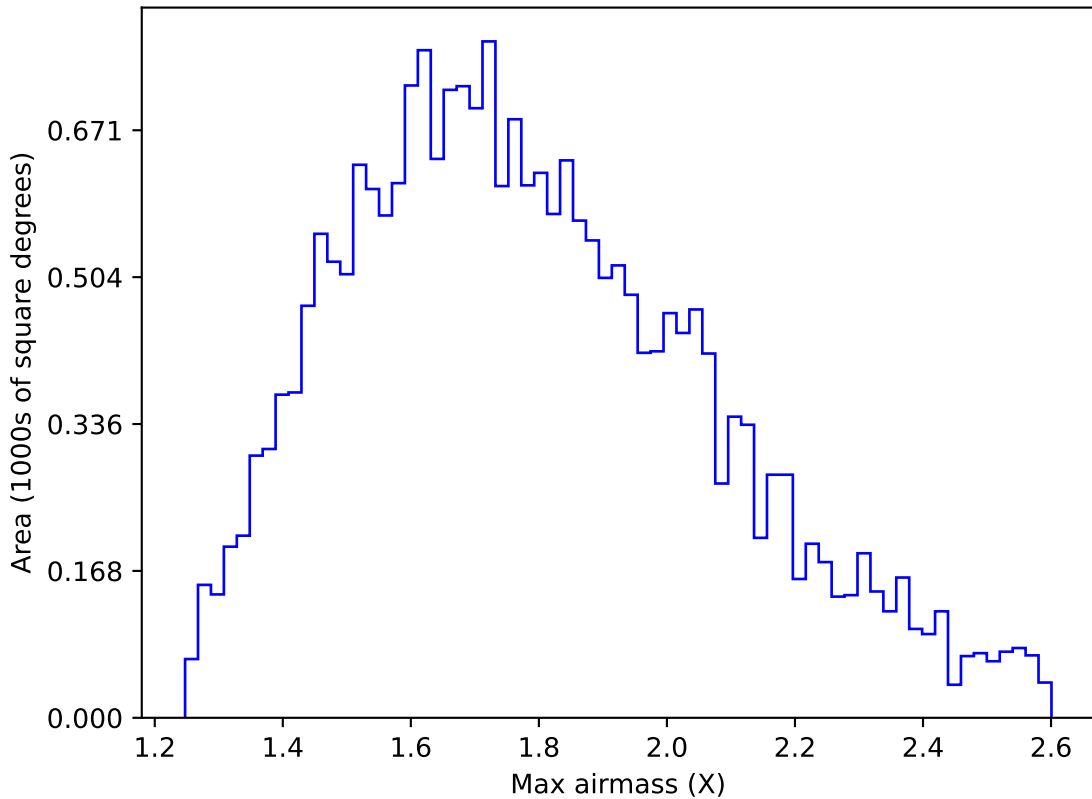
too_ignore_100_4v3.4_10yrs All sky u band: Max airmass
