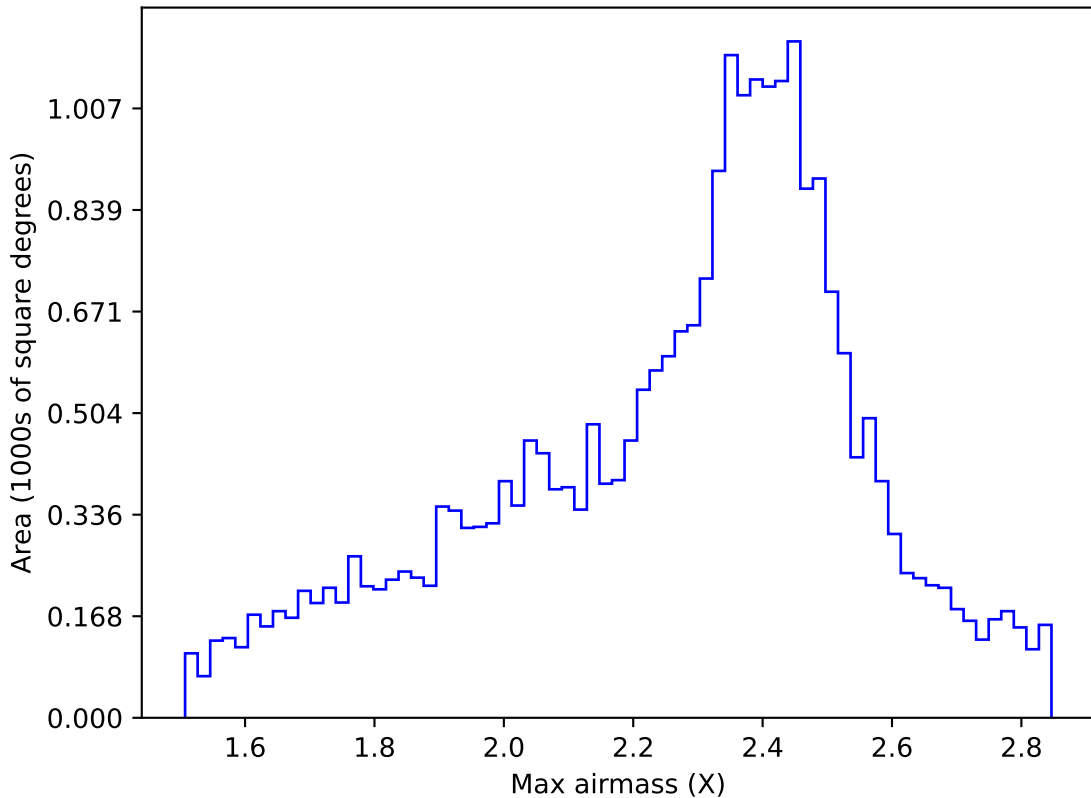
too_ignore_100_4v3.4_10yrs All sky r band: Max airmass
