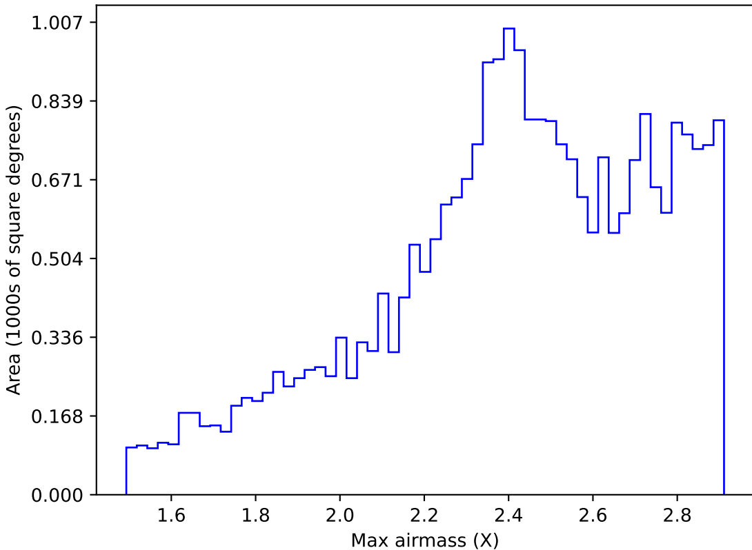
too_ignore_100_4v3.4_10yrs All sky i band: Max airmass
