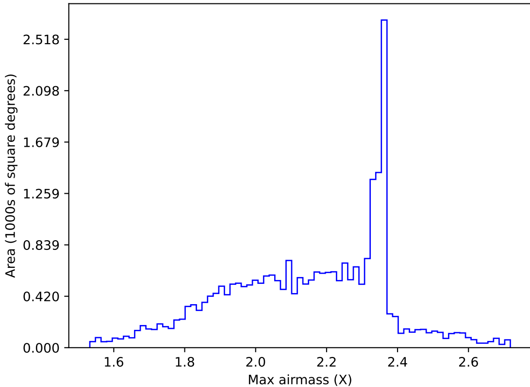
too_ignore_100_4v3.4_10yrs All sky g band: Max airmass
