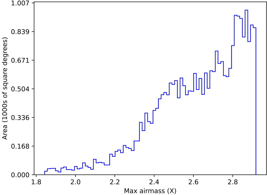
too_ignore_100_4v3.4_10yrs All sky all bands: Max airmass
