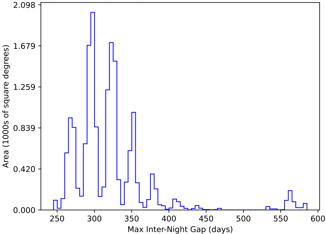
too_ignore_100_4v3.4_10yrs WFD y band: Max Inter-Night Gap
