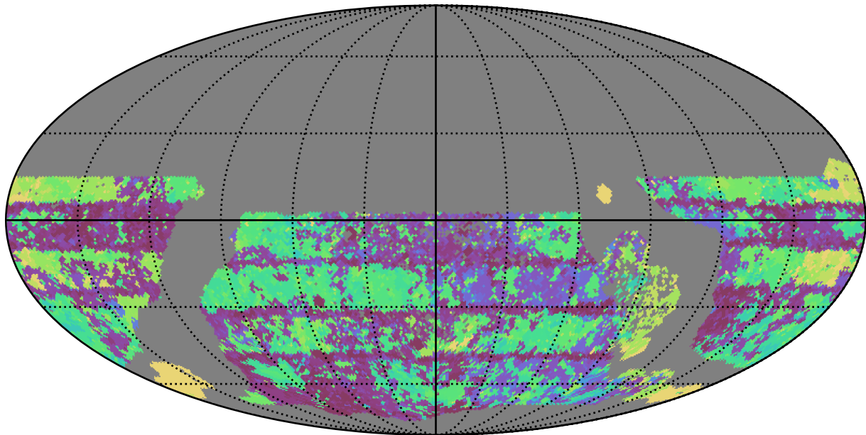
too_ignore_100_4v3.4_10yrs WFD u band: Max Inter-Night Gap
