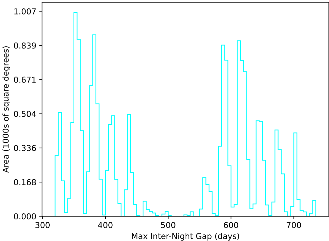
too_ignore_100_4v3.4_10yrs WFD u band: Max Inter-Night Gap
