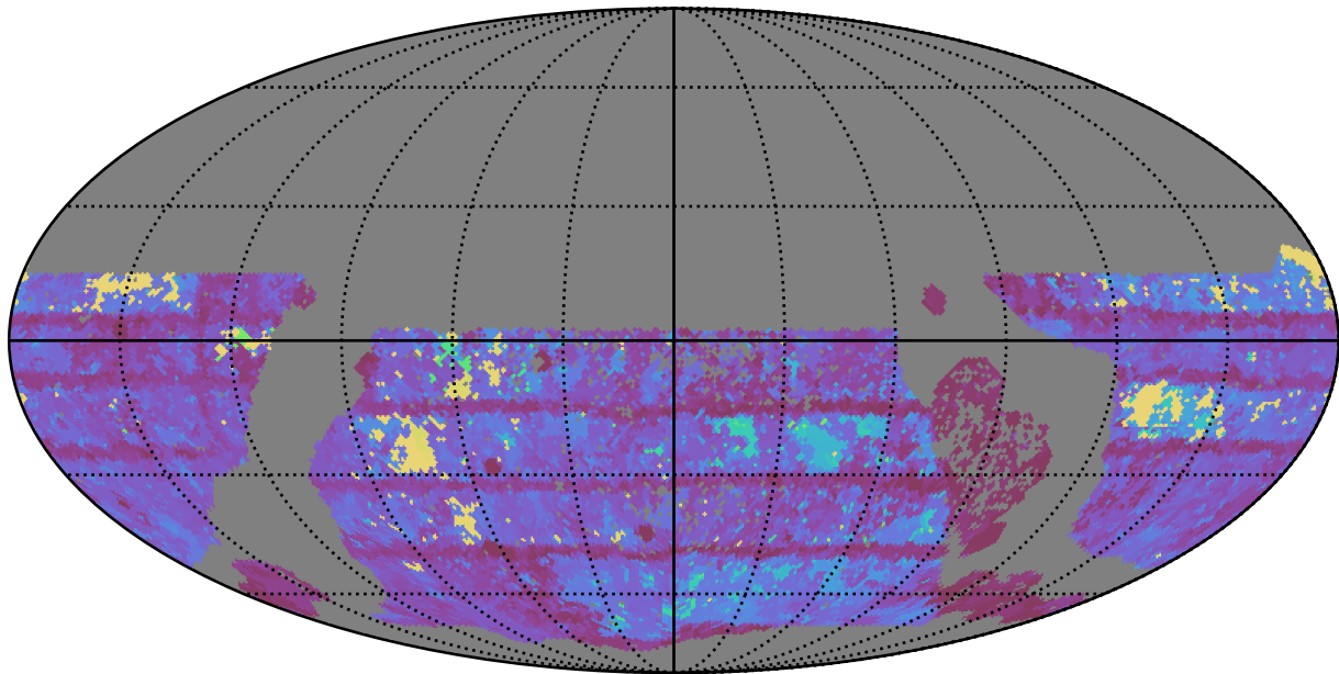
too_ignore_100_4v3.4_10yrs WFD r band: Max Inter-Night Gap
