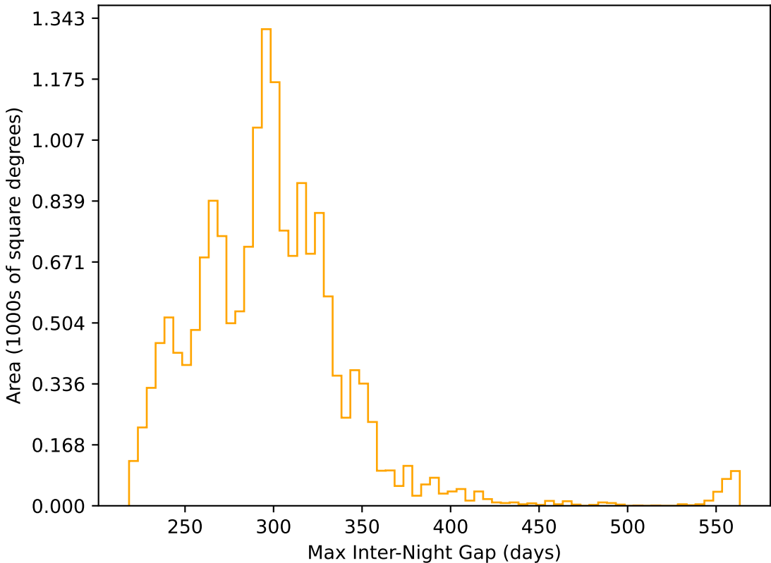
too_ignore_100_4v3.4_10yrs WFD r band: Max Inter-Night Gap
