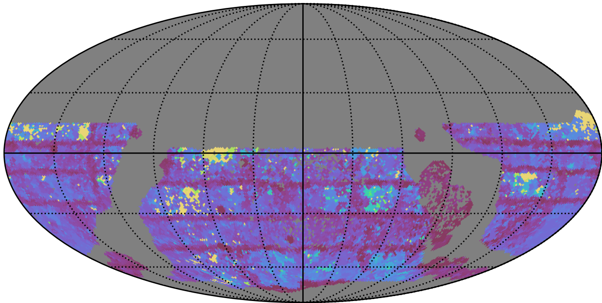
too_ignore_100_4v3.4_10yrs WFD i band: Max Inter-Night Gap
