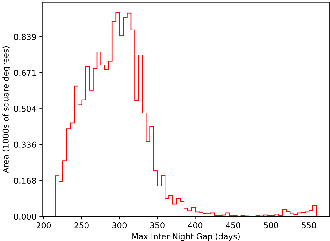
too_ignore_100_4v3.4_10yrs WFD i band: Max Inter-Night Gap
