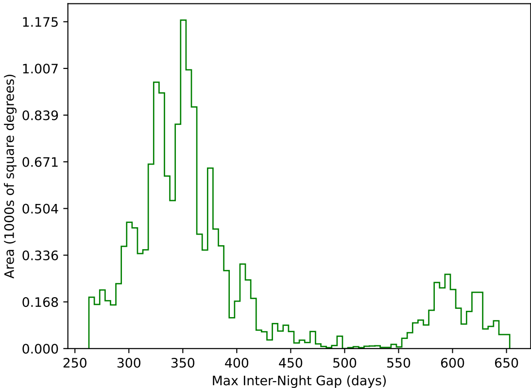
too_ignore_100_4v3.4_10yrs WFD g band: Max Inter-Night Gap
