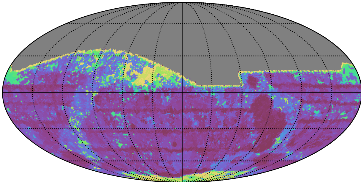
too_ignore_100_4v3.4_10yrs All sky z band: Max Inter-Night Gap
