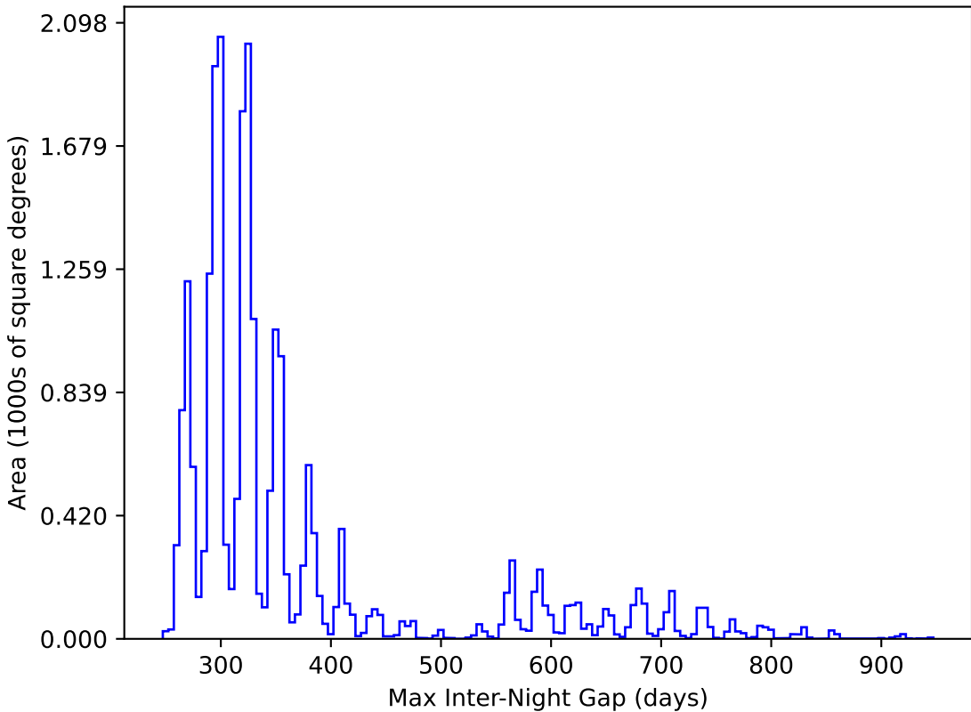
too_ignore_100_4v3.4_10yrs All sky y band: Max Inter-Night Gap
