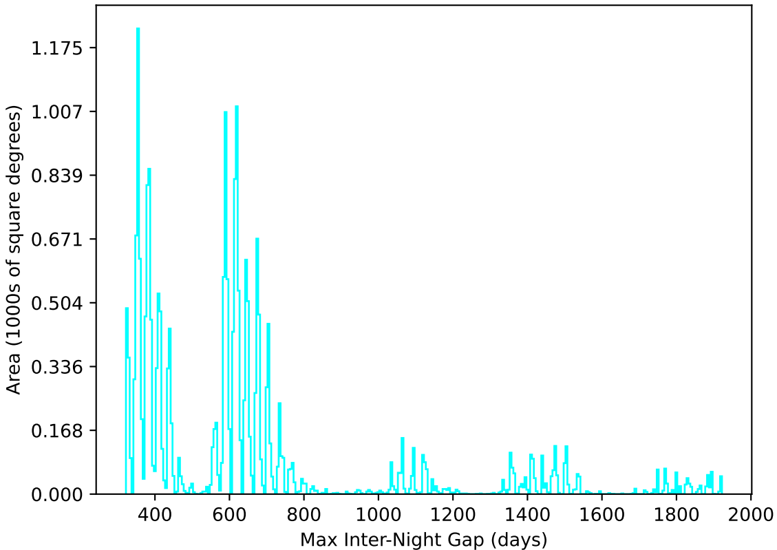
too_ignore_100_4v3.4_10yrs All sky u band: Max Inter-Night Gap
