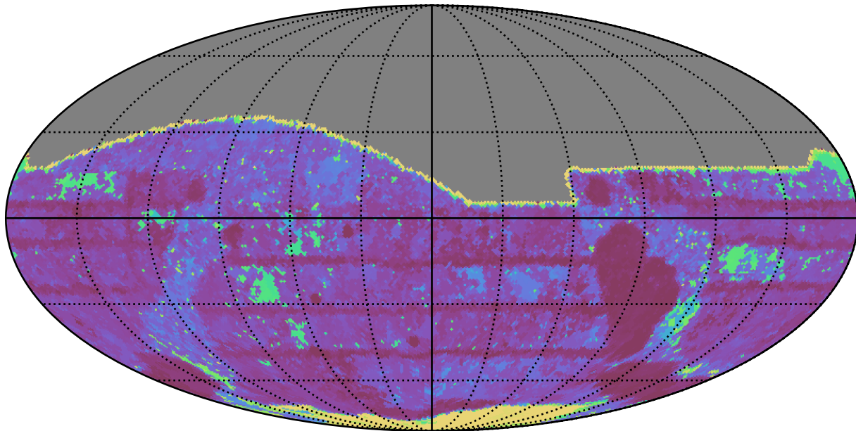
too_ignore_100_4v3.4_10yrs All sky r band: Max Inter-Night Gap
