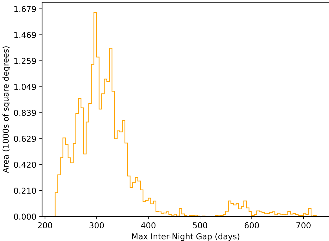
too_ignore_100_4v3.4_10yrs All sky r band: Max Inter-Night Gap
