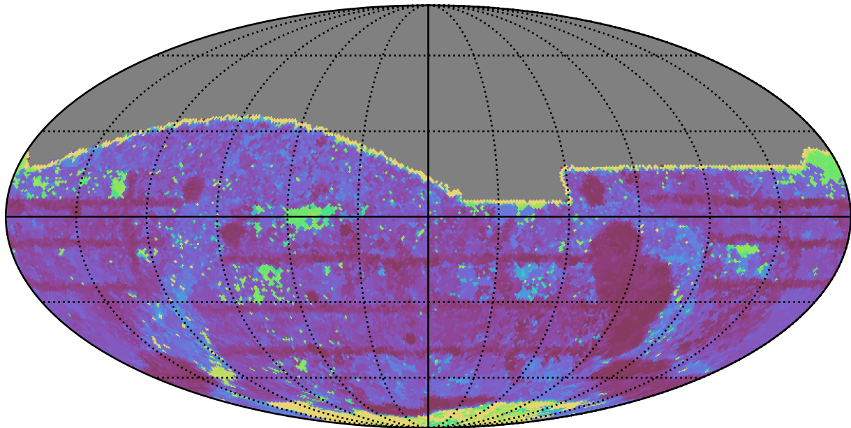
too_ignore_100_4v3.4_10yrs All sky i band: Max Inter-Night Gap
