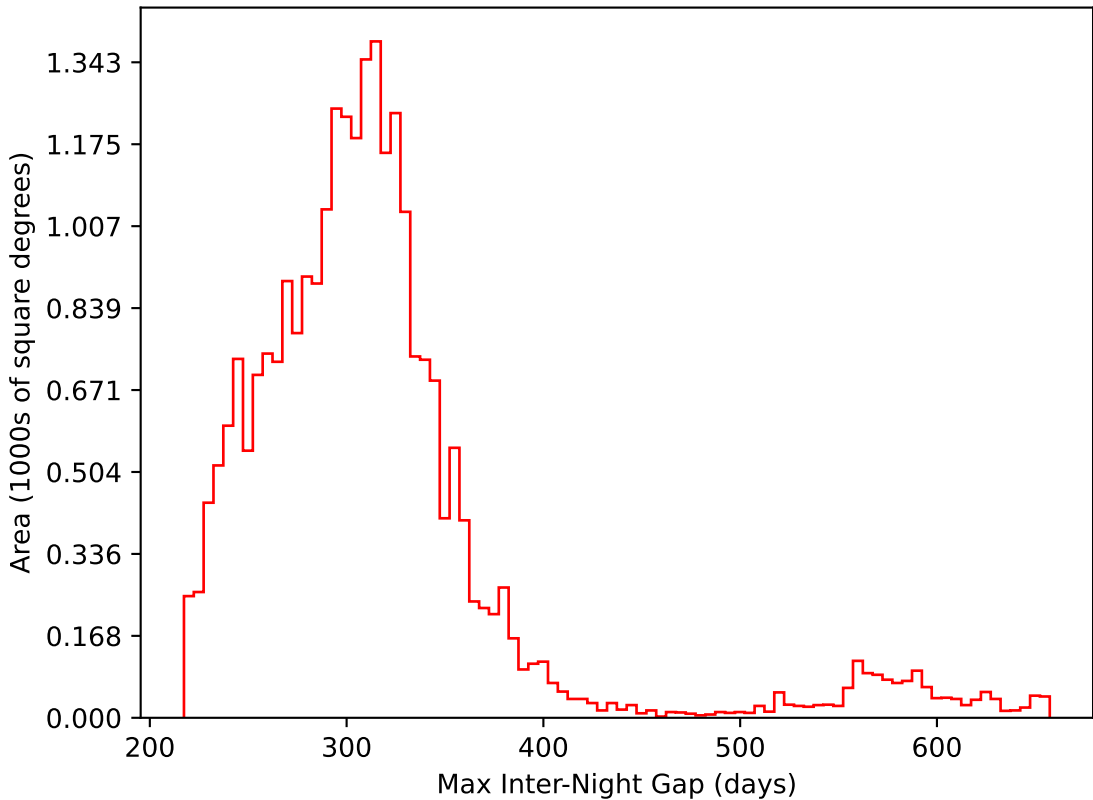
too_ignore_100_4v3.4_10yrs All sky i band: Max Inter-Night Gap
