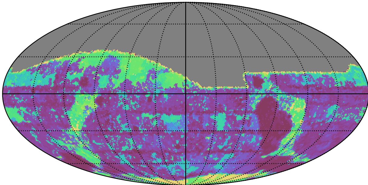
too_ignore_100_4v3.4_10yrs All sky g band: Max Inter-Night Gap
