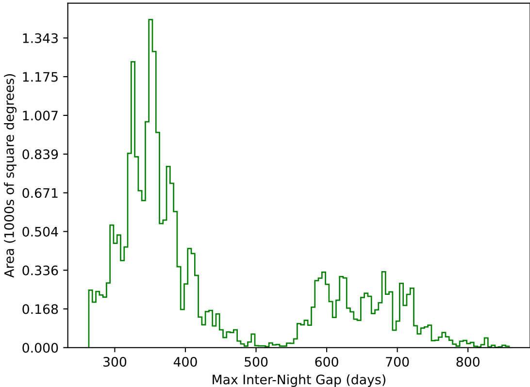
too_ignore_100_4v3.4_10yrs All sky g band: Max Inter-Night Gap
