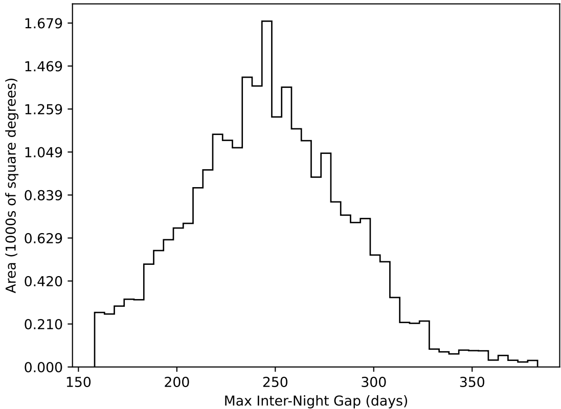
too_ignore_100_4v3.4_10yrs All sky all bands: Max Inter-Night Gap
