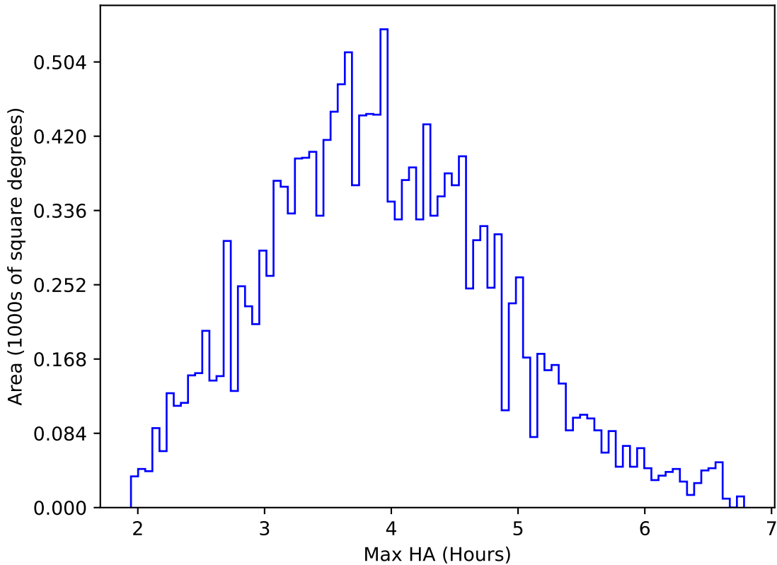
too_ignore_100_4v3.4_10yrs WFD u band: Max HA
