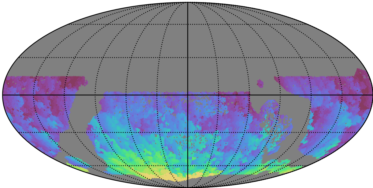
too_ignore_100_4v3.4_10yrs WFD r band: Max HA
