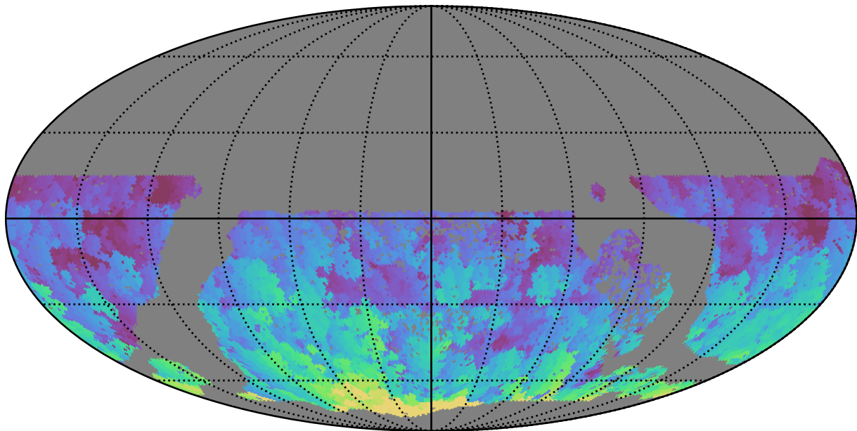
too_ignore_100_4v3.4_10yrs WFD g band: Max HA
