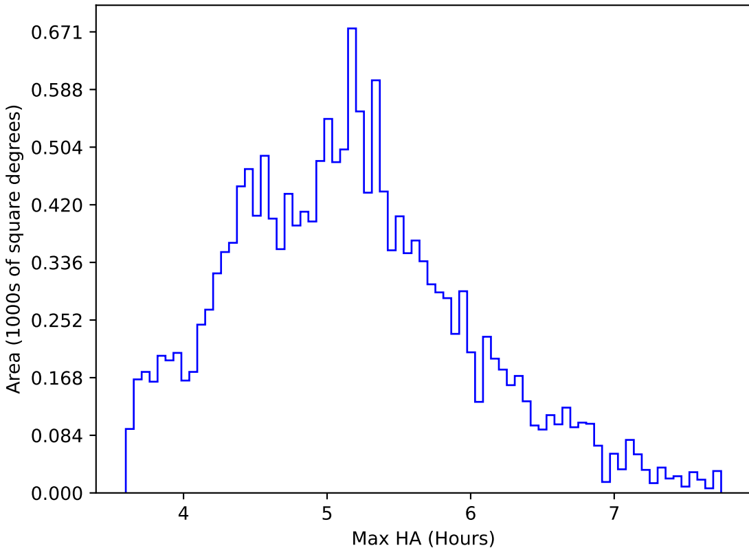
too_ignore_100_4v3.4_10yrs WFD all bands: Max HA
