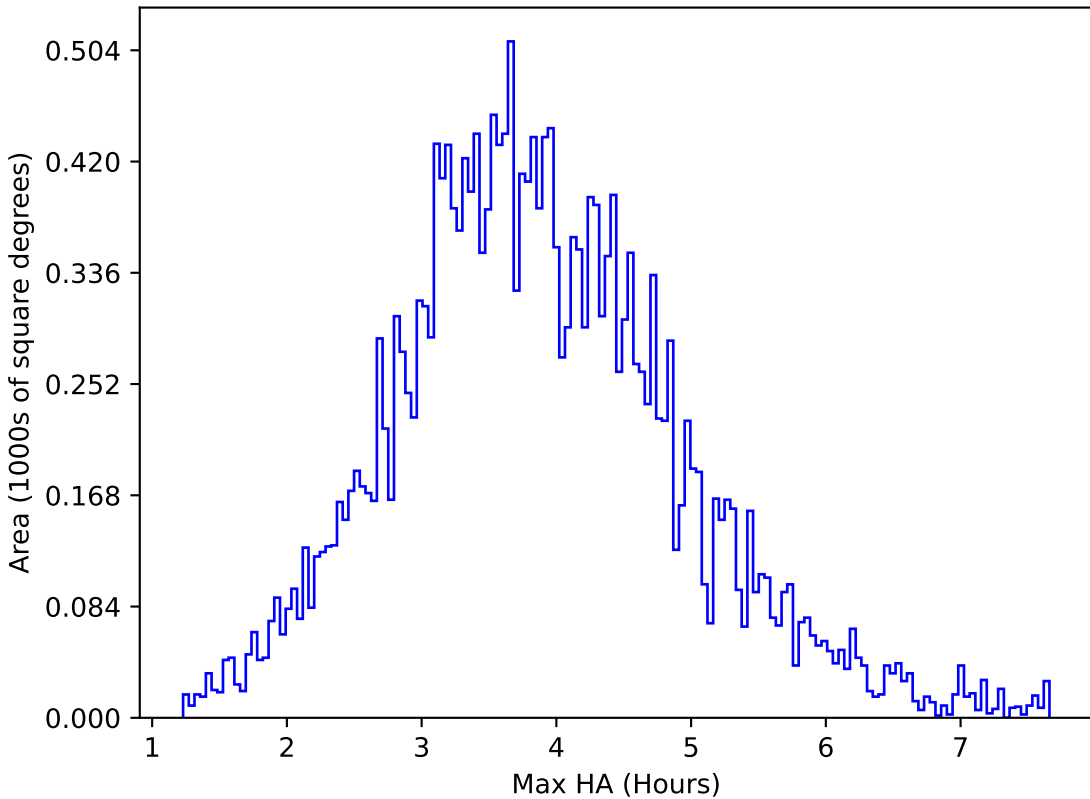
too_ignore_100_4v3.4_10yrs All sky u band: Max HA
