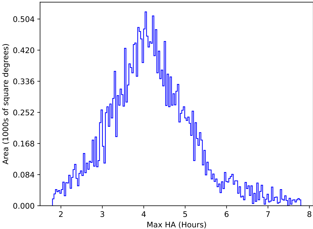
too_ignore_100_4v3.4_10yrs All sky r band: Max HA
