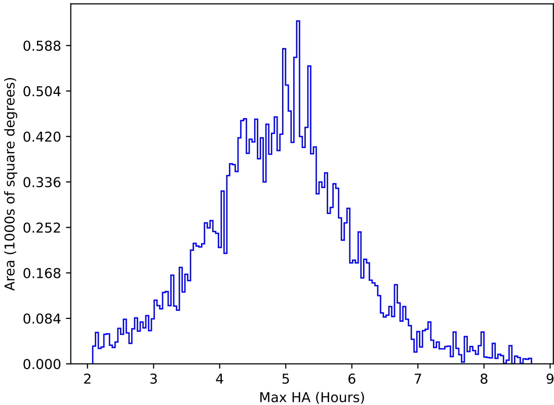
too_ignore_100_4v3.4_10yrs All sky all bands: Max HA
