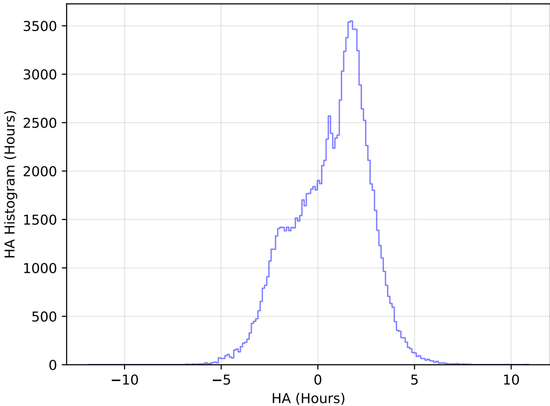
too_ignore_100_4v3.4_10yrs WFD u band: HA Histogram
