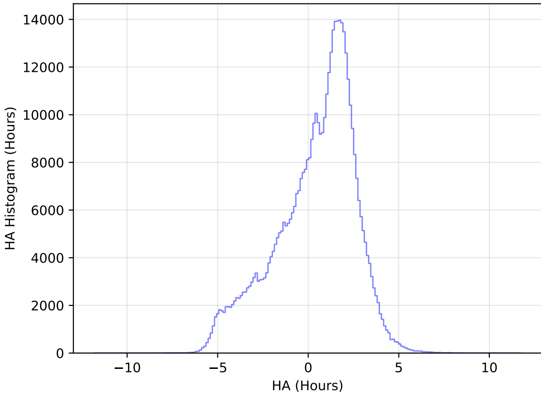
too_ignore_100_4v3.4_10yrs WFD r band: HA Histogram
