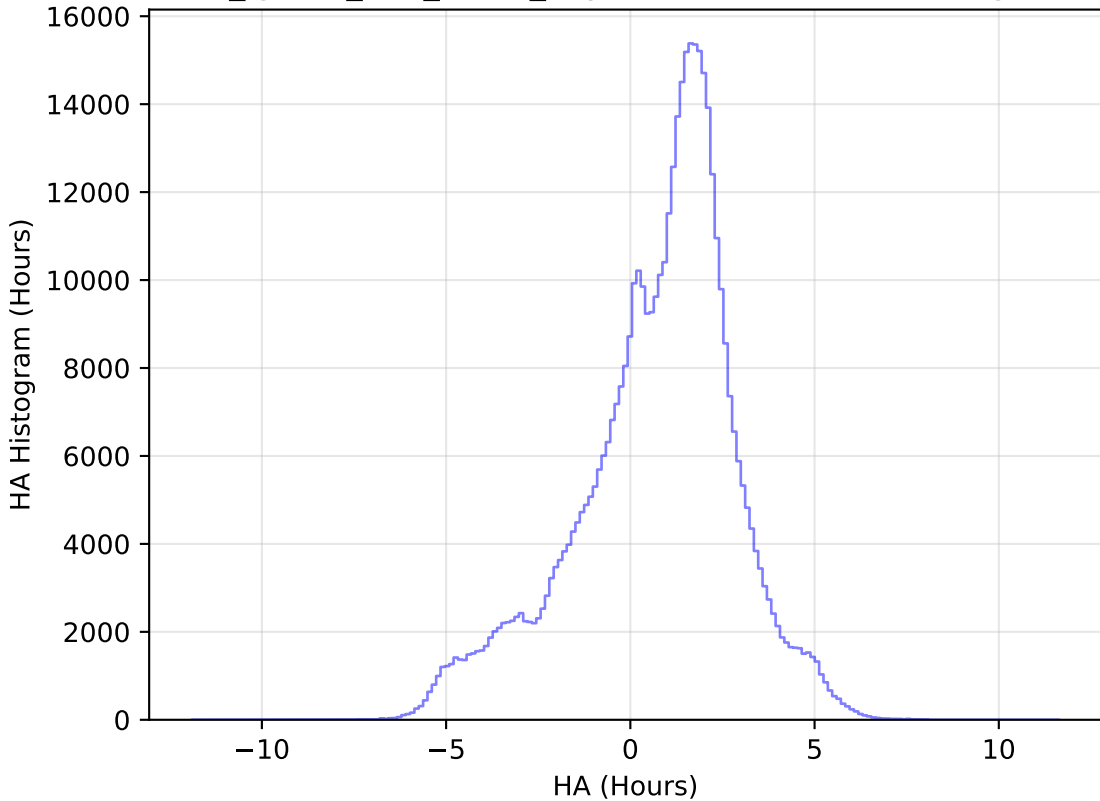
too_ignore_100_4v3.4_10yrs WFD i band: HA Histogram
