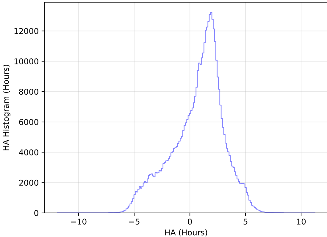
too_ignore_100_4v3.4_10yrs All sky z band: HA Histogram
