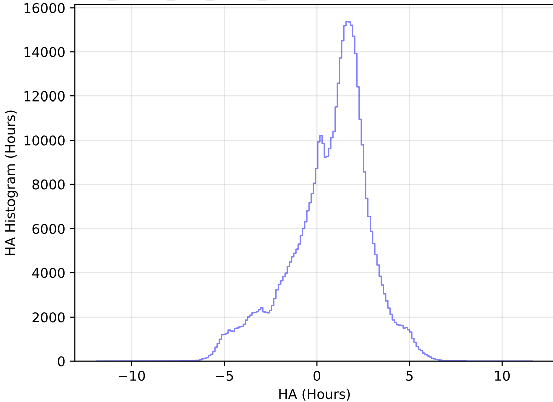
too_ignore_100_4v3.4_10yrs All sky i band: HA Histogram
