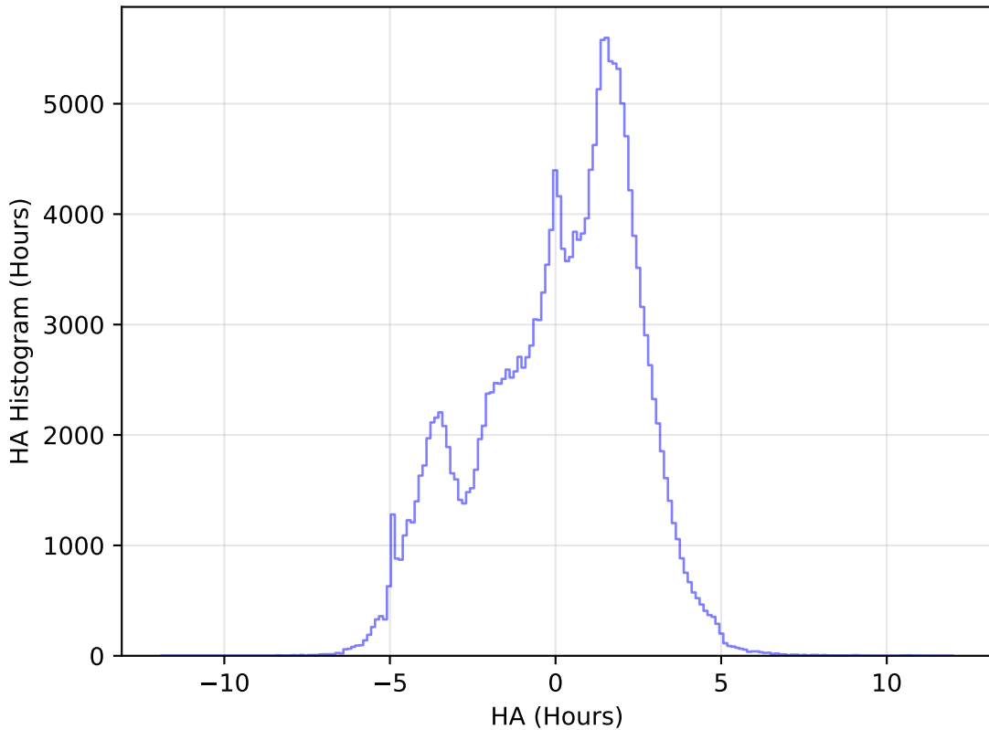
too_ignore_100_4v3.4_10yrs All sky g band: HA Histogram
