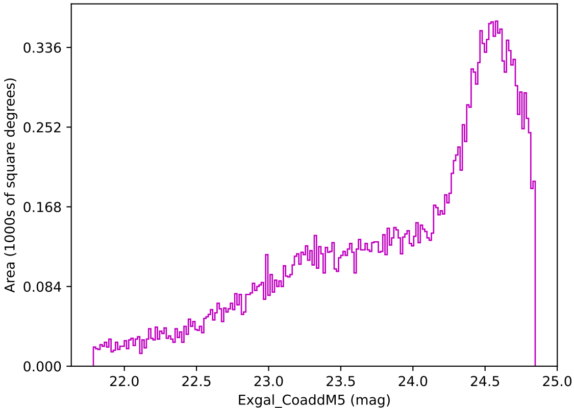
too_ignore_100_4v3.4_10yrs Yr 3-4 z band: Exgal_CoaddM5
