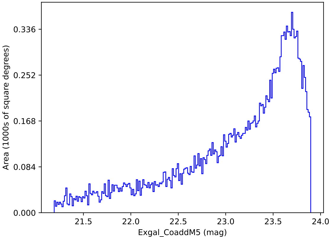
too_ignore_100_4v3.4_10yrs Yr 3-4 y band: Exgal_CoaddM5
