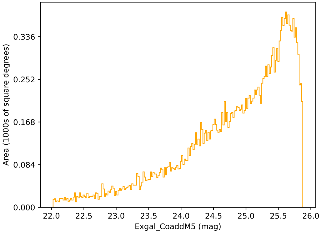
too_ignore_100_4v3.4_10yrs Yr 3-4 r band: Exgal_CoaddM5
