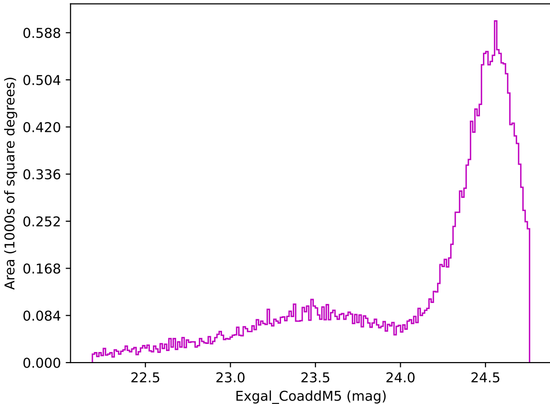
too_ignore_100_4v3.4_10yrs Yr 1 z band: Exgal_CoaddM5
