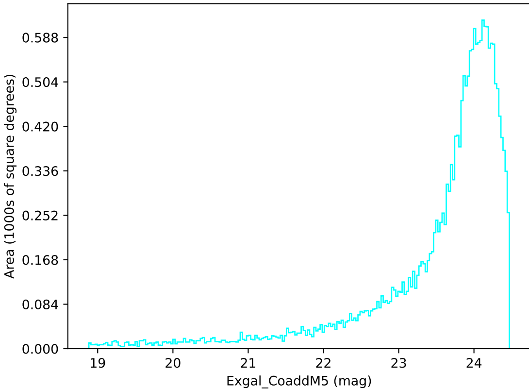
too_ignore_100_4v3.4_10yrs Yr 1 u band: Exgal_CoaddM5
