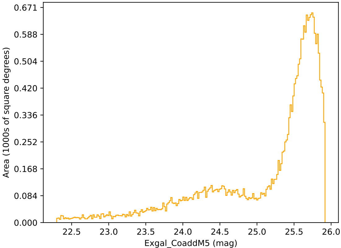
too_ignore_100_4v3.4_10yrs Yr 1 r band: Exgal_CoaddM5
