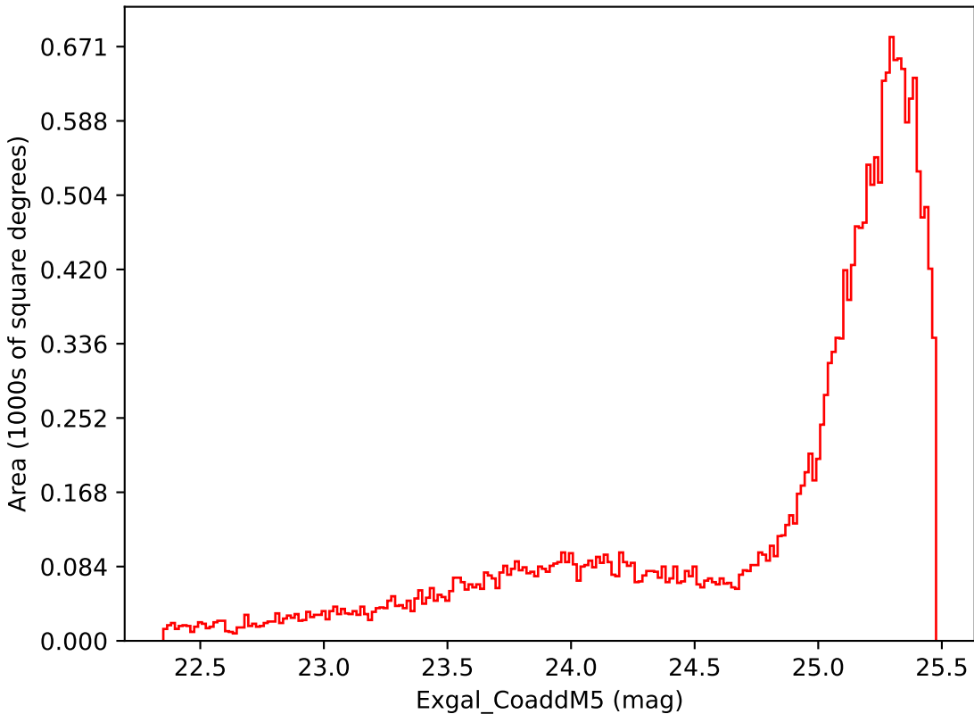
too_ignore_100_4v3.4_10yrs Yr 1 i band: Exgal_CoaddM5
