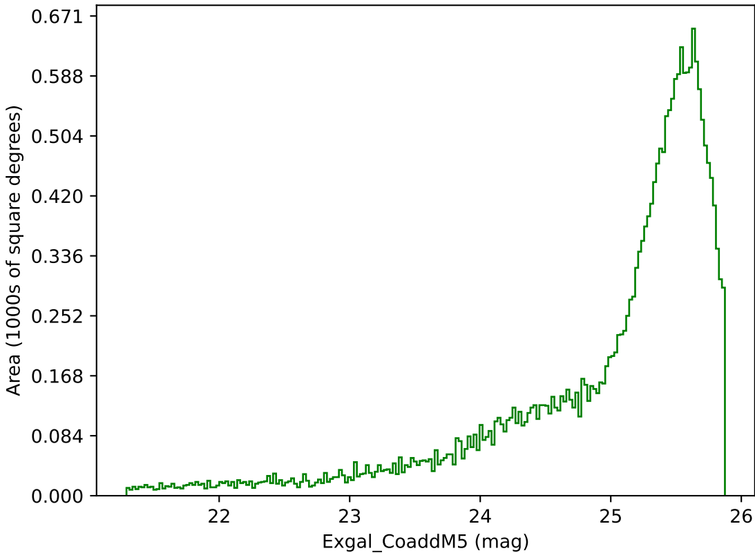
too_ignore_100_4v3.4_10yrs Yr 1 g band: Exgal_CoaddM5
