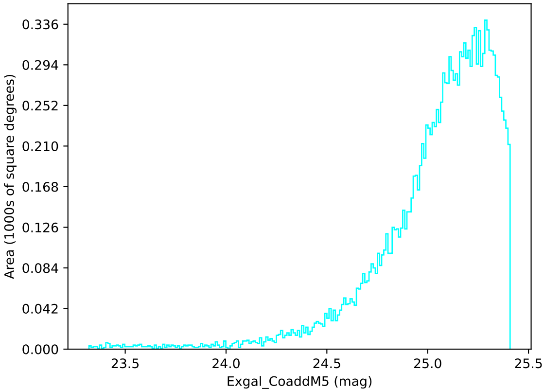
too_ignore_100_4v3.4_10yrs WFD u band: Exgal_CoaddM5
