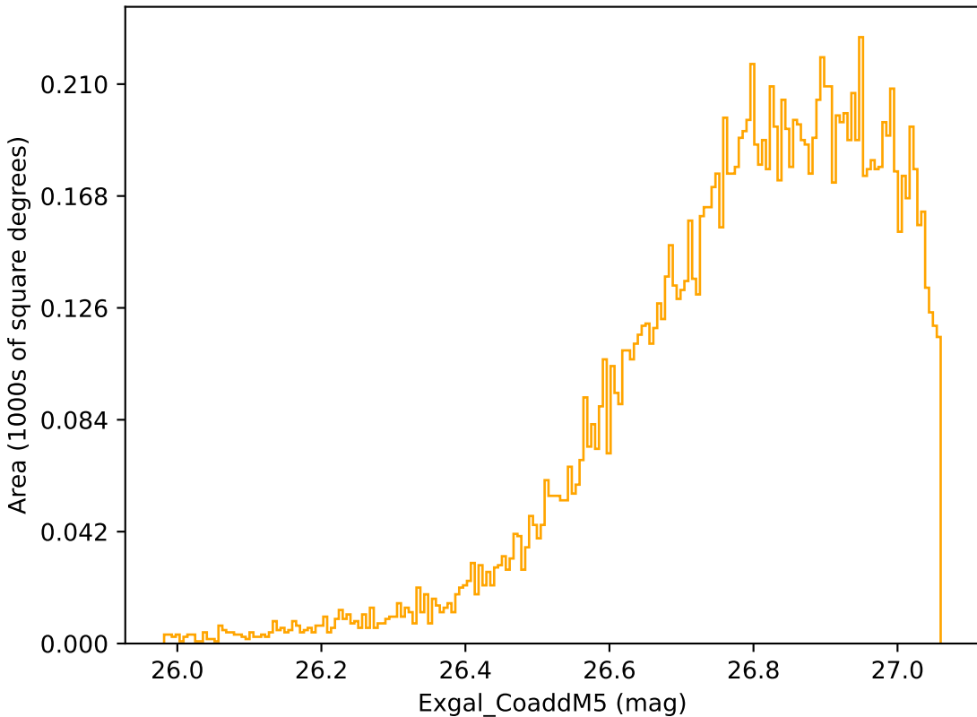
too_ignore_100_4v3.4_10yrs WFD r band: Exgal_CoaddM5
