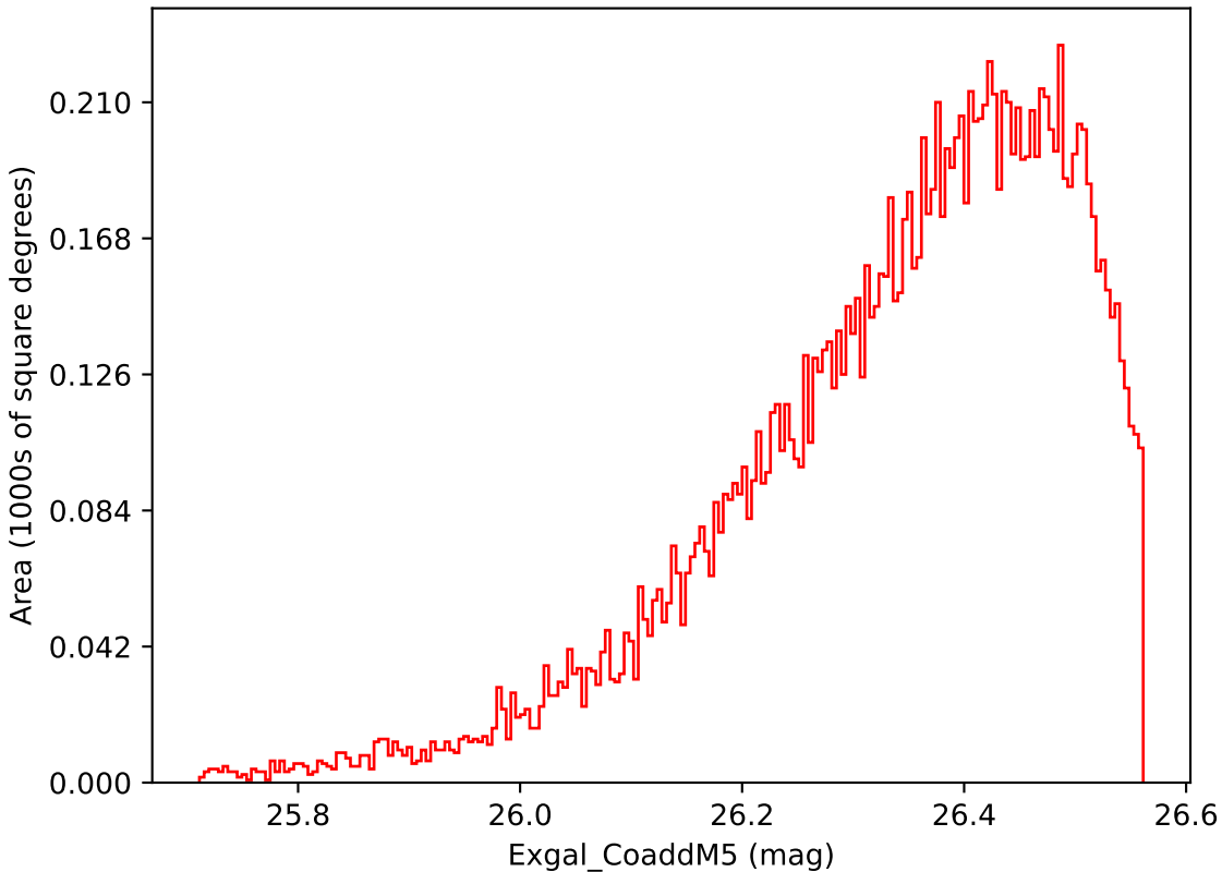
too_ignore_100_4v3.4_10yrs WFD i band: Exgal_CoaddM5
