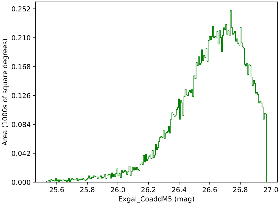
too_ignore_100_4v3.4_10yrs WFD g band: Exgal_CoaddM5
